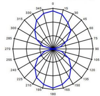
Orientation Sensitivity
